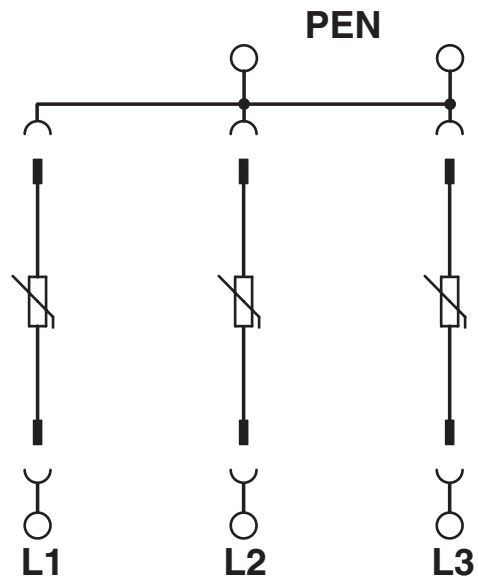
Circuit diagram
