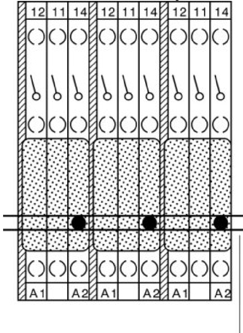
Dimensional drawing
