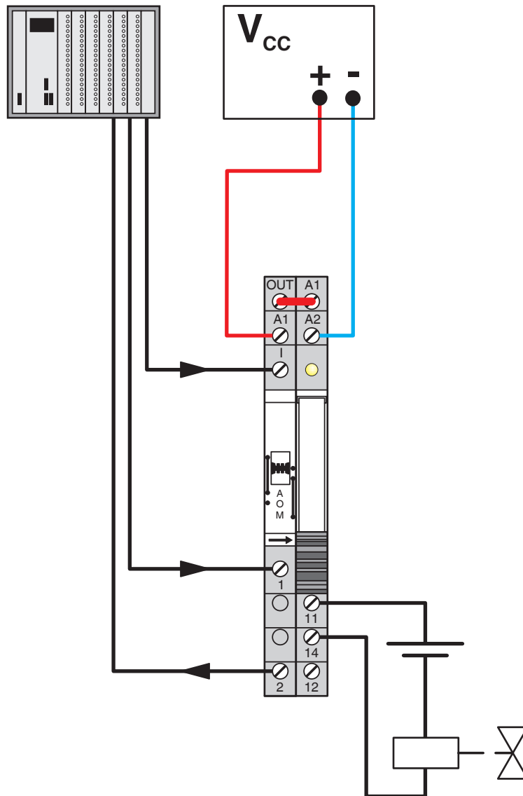
Application drawing
