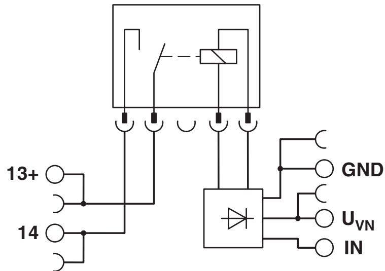
Circuit diagram
