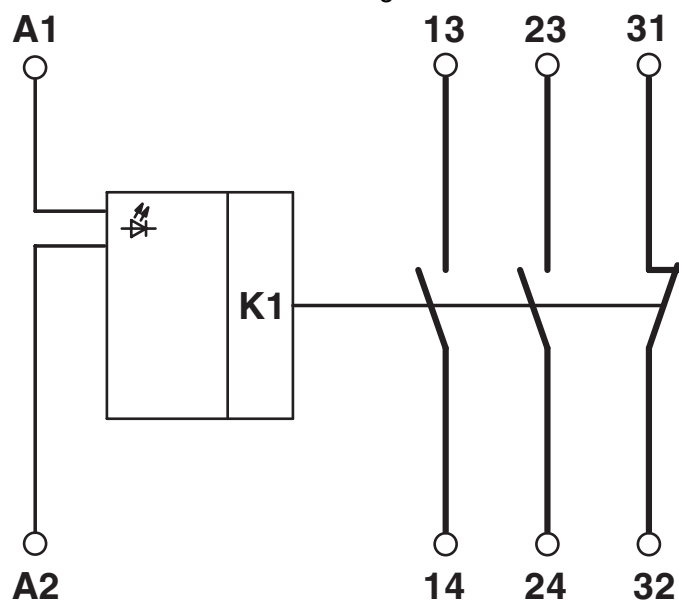
Circuit diagram
