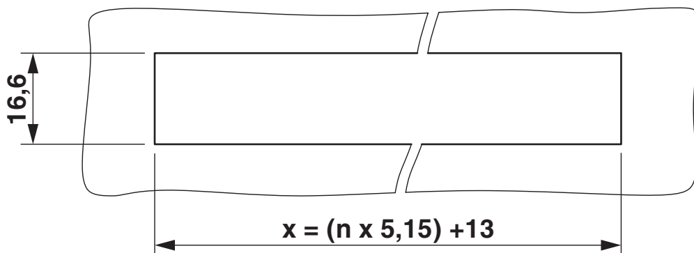
Dimensional drawing
