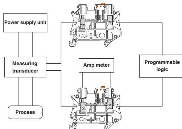
Application drawing
