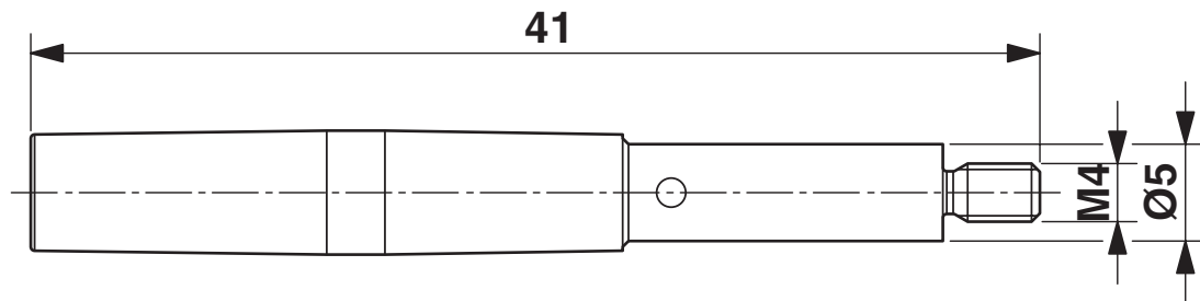
Dimensional drawing
