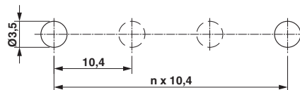
Dimensional drawing
