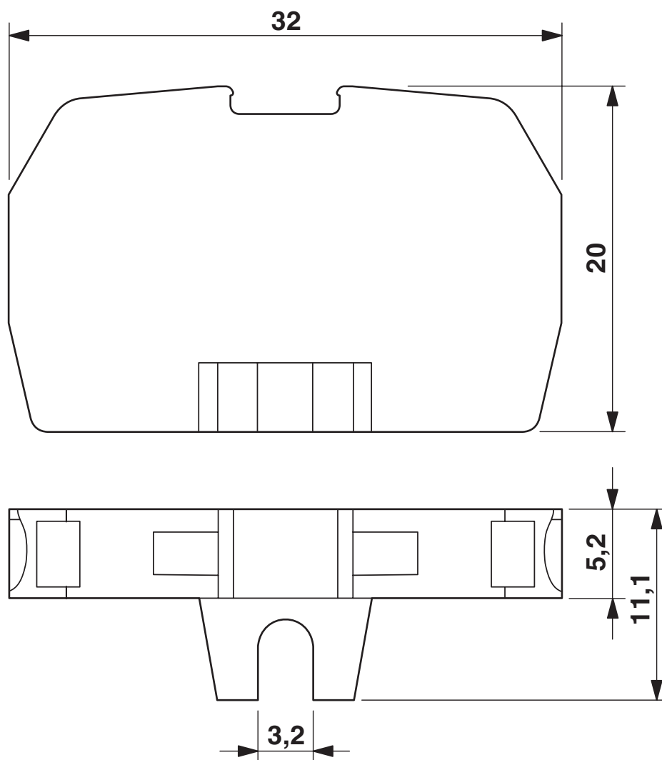
Dimensional drawing
