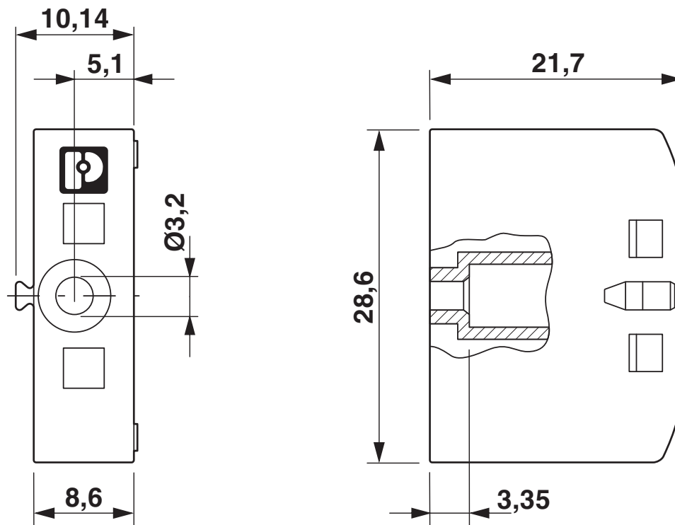
Dimensional drawing
