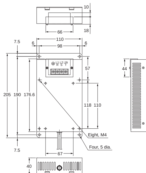
3G3AX-EFIB2 3G3AX-EFI22
