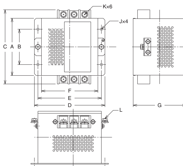
3G3AX-NFO03/3G3AX-NFO04/3G3AX-NFO05 3G3AX-NFO06/3G3AX-NFO07
