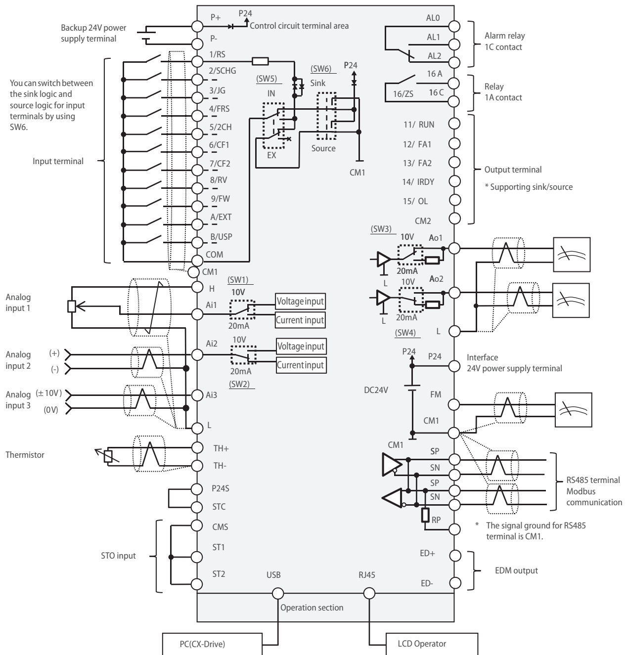
Control circuit
