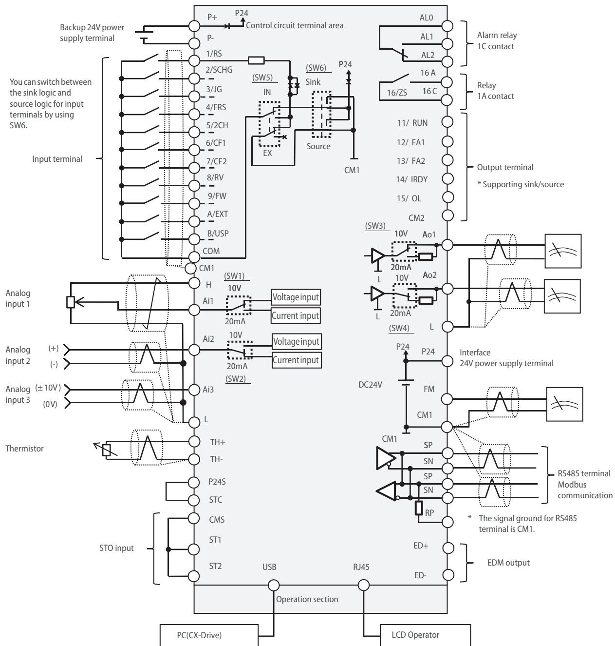
Control circuit
