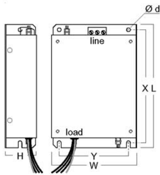
Dimension diagram 1
