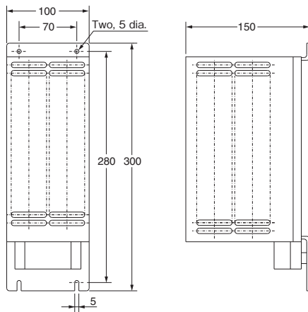
3G3AX-RBB4001
