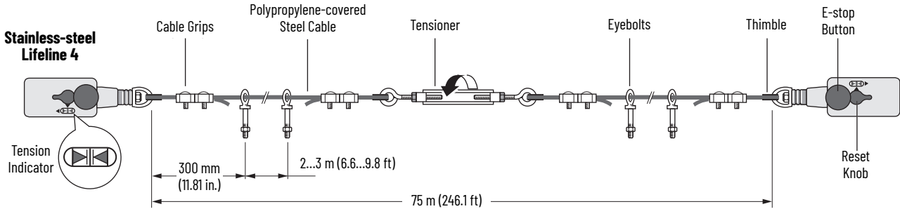
Figure 5 - Spring Tensioner
