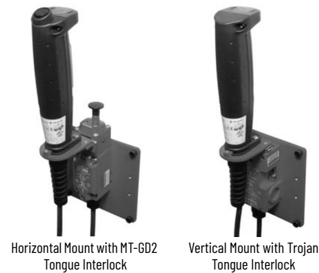
Figure 18 - Single-switch Mounting
