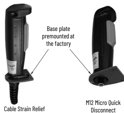
Figure 13 - 440J Enabling Switch with Base Plate
