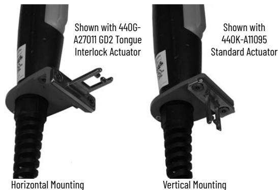
Figure 16 - Horizontal and Vertical Mounting
