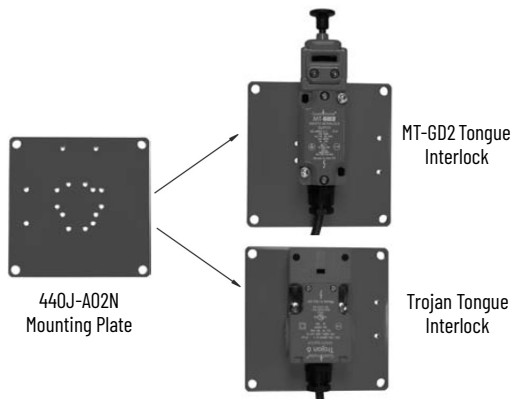
Figure 17 - Mounting Plate
