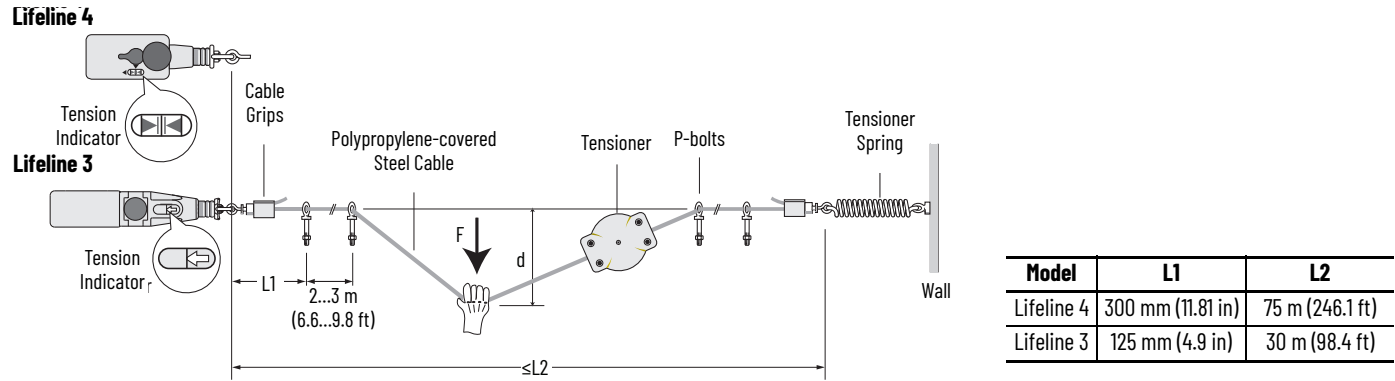
Figure 5 - Spring Tensioner
