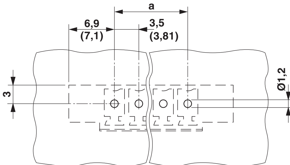
Dimensional drawing
