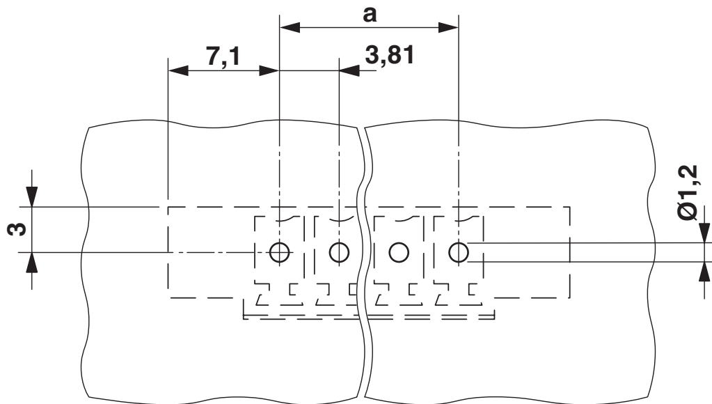
Dimensional drawing
