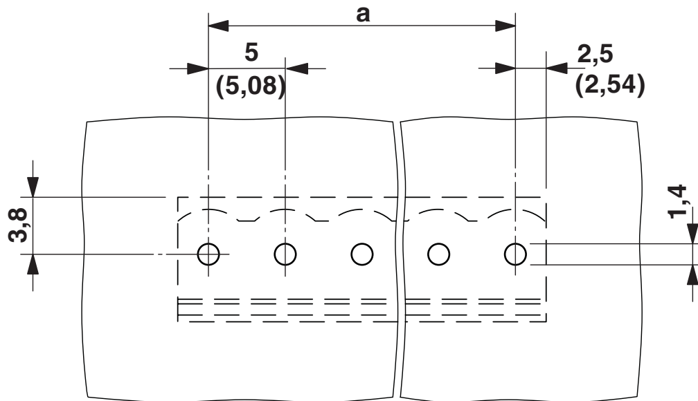
Dimensional drawing
