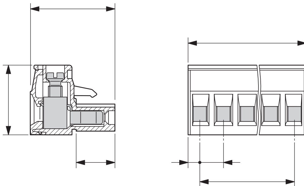
Dimensional drawing
