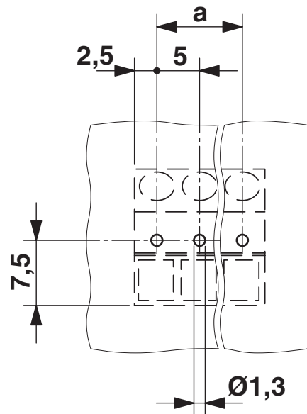
Dimensional drawing
