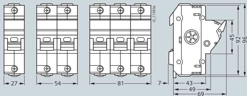
3NC1 491/3NC1 492/3NC1 493
