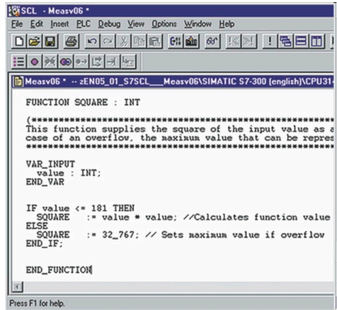
Declaration and instruction part of a function block in S7-SCL
