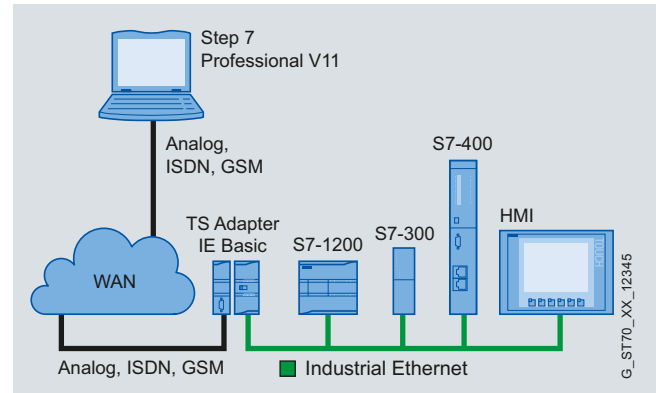
System configuration for remote maintenance. A programming device/PC is not required on the plant side. Connection is made direct to PROFINET. Routing enables access across network boundaries.
