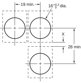
Panel Cutout (Top View)
