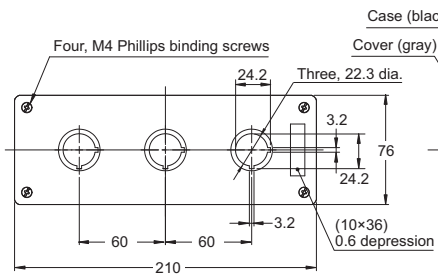
Control Box (3 holes) A22NZ-A-B103
