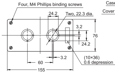
Control Box (2 holes) A22NZ-A-B102
