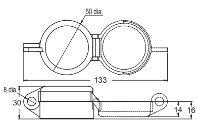
Plastic Hole Plug A22NZ-A-401
