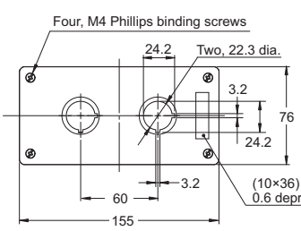
Control Box (2 holes) A22NZ-A-B102
