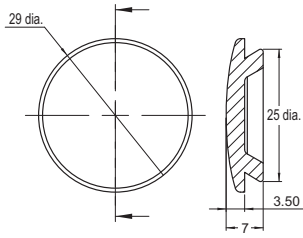
Plastic Hole Plug A22NZ-A-401
