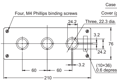
Control Box (3 holes) A22NZ-A-B103
