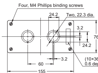
Control Box (2 holes) A22NZ-A-B102
