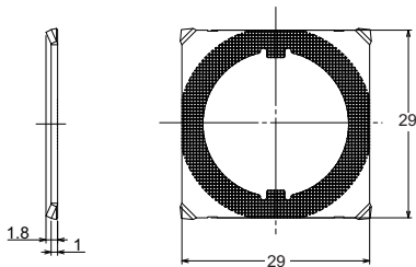
Reinforcement Plate A22NZ-A-C01
