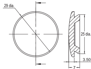
Plastic Hole Plug A22NZ-A-401
