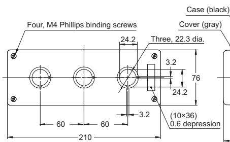
Control Box (3 holes) A22NZ-A-B103
