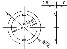
OGL-11 Anti-Rotation Ring
