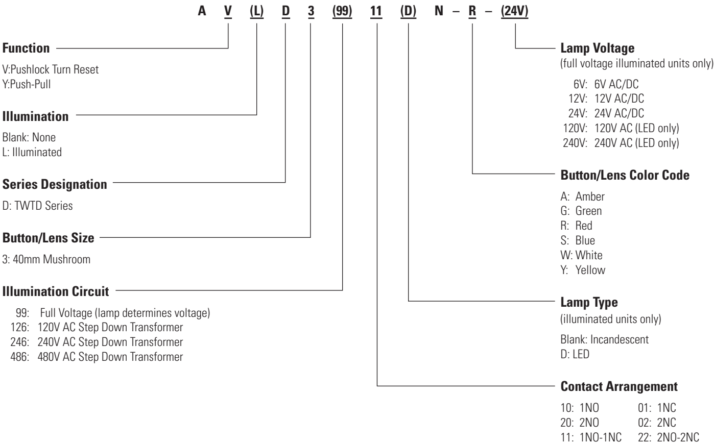
Assembled Stop Switches
