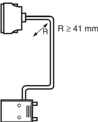
CS1 to C200H I/O Connecting Cable (Cable diameter: 5.1 mm)
