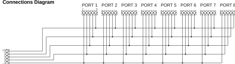
Connections Diagram
