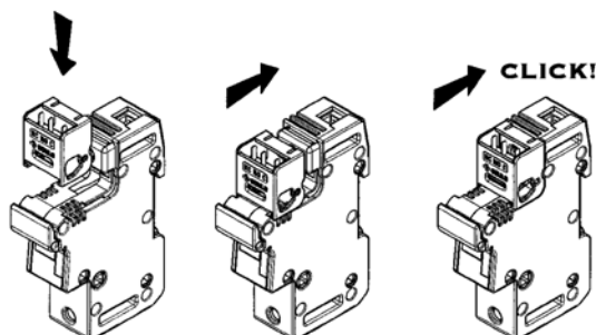
1- assembly
