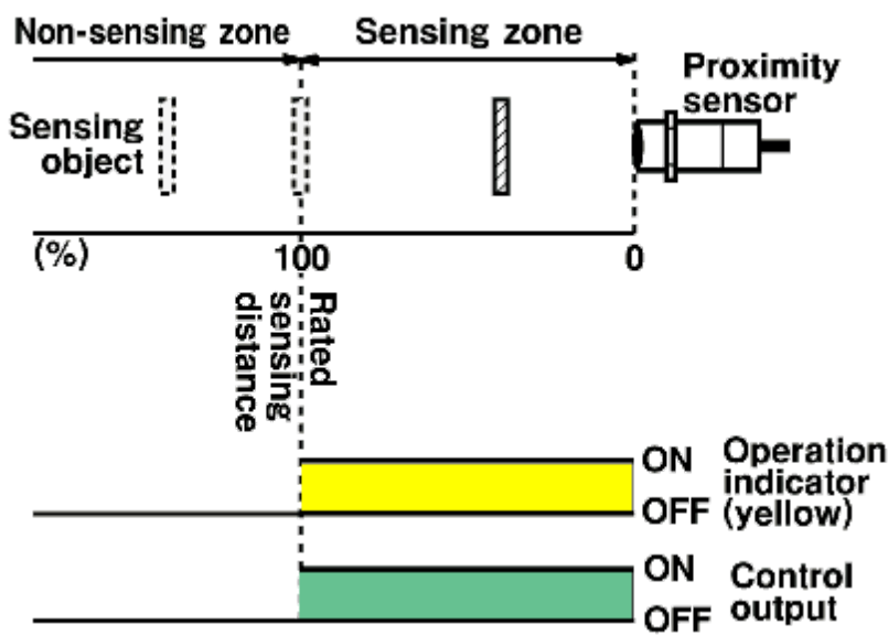
Timing chart
