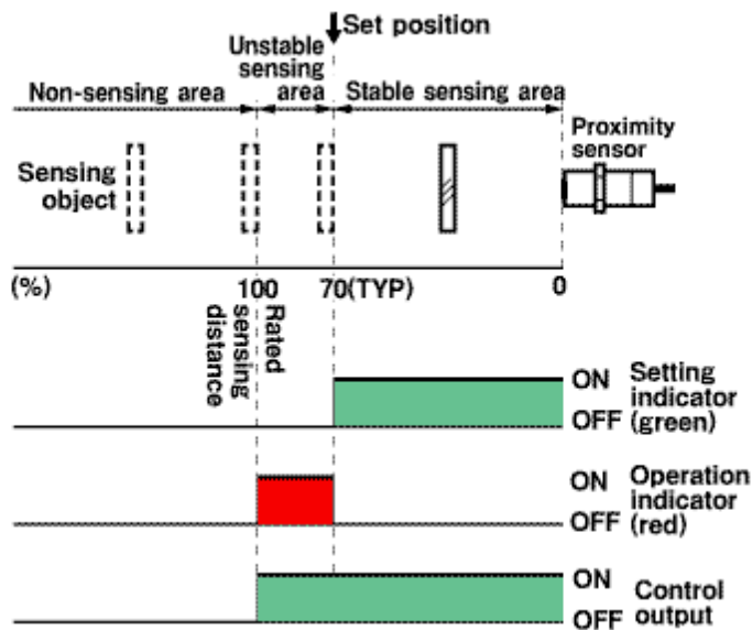
Timing chart
