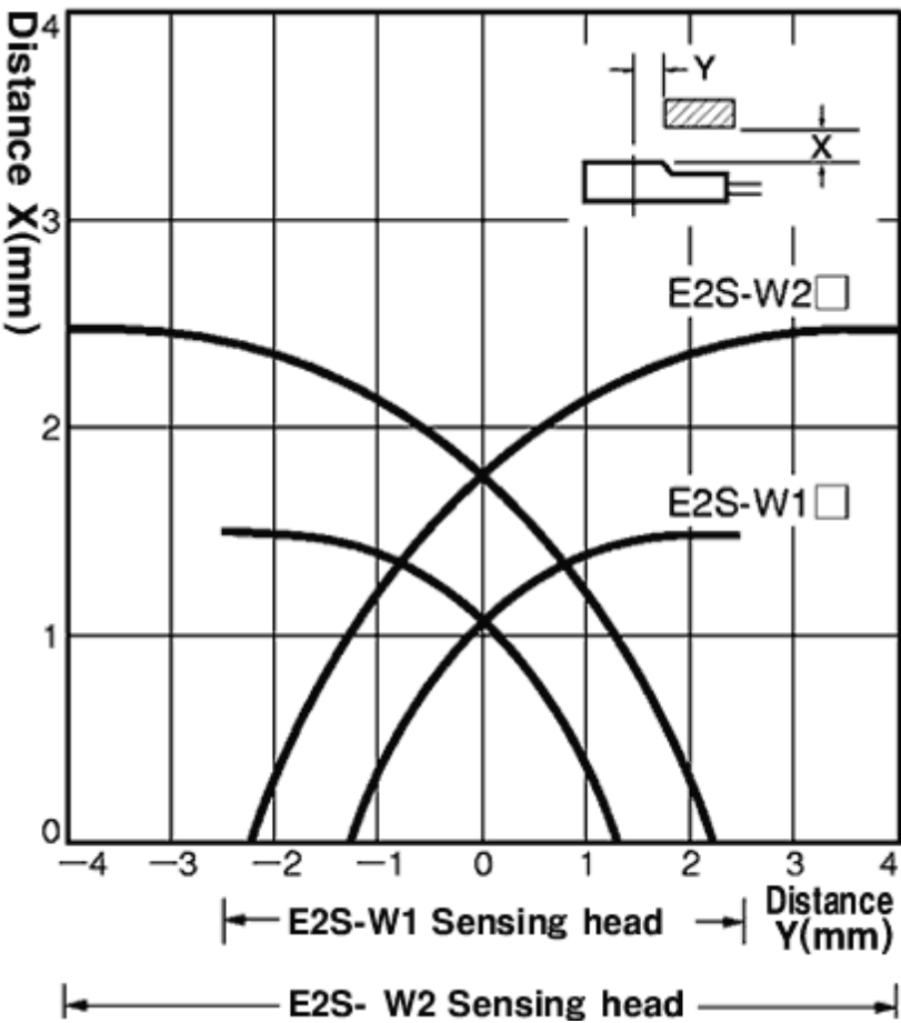
Sensing range
