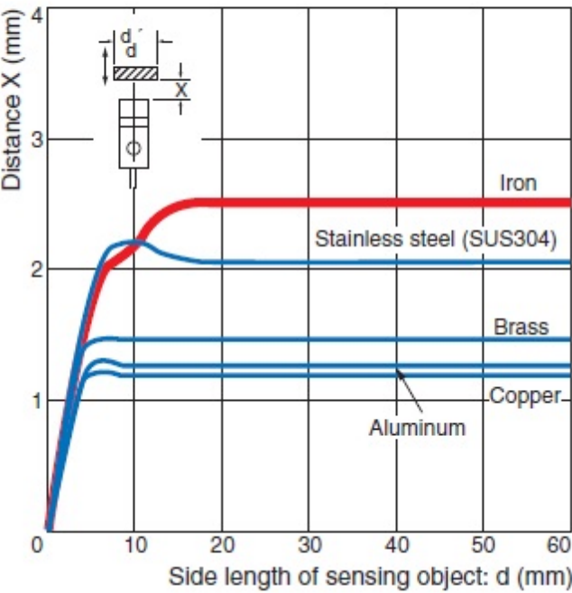
Sensing range
