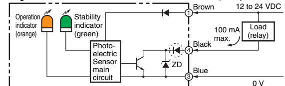
Protection for NPN output models
