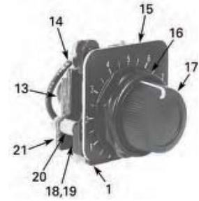
Potentiometers
