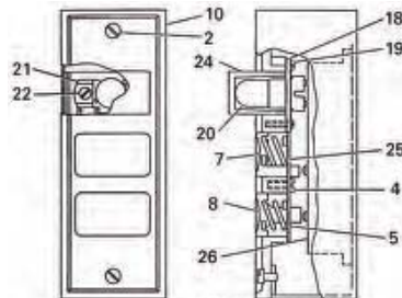
Two Element Station with Indicating Light
