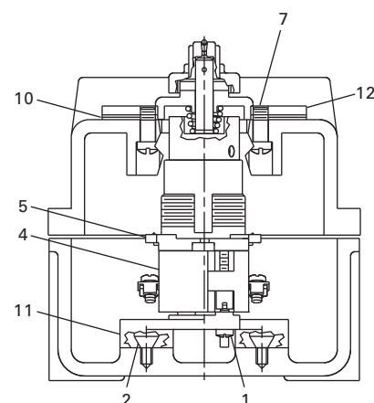
Selector Switch
