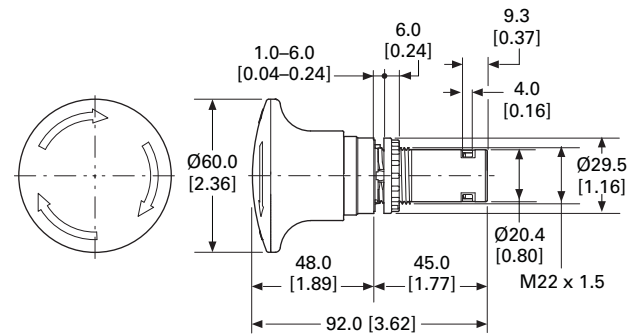
C22-PVT60P_
