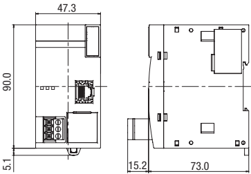
FC6A-EXM1S
