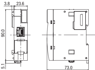
FC6A-EXM1M
