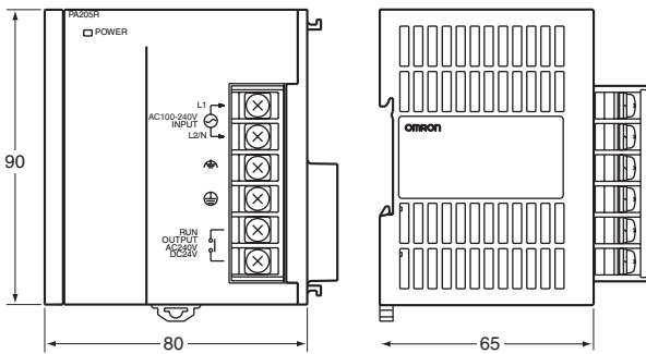
Power Supply Units CJ1W-PA205R
