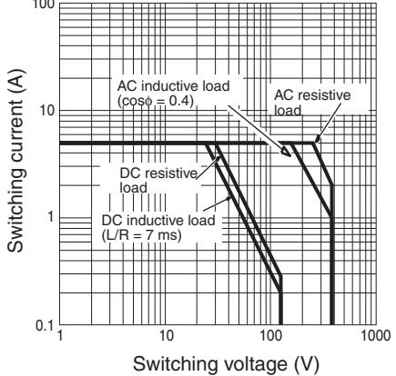
G2R-2-S (S)
