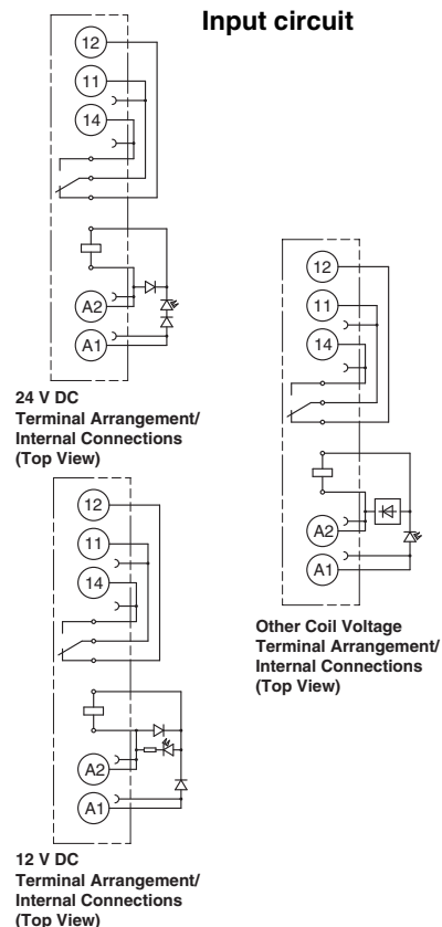
Terminal Arrangement
