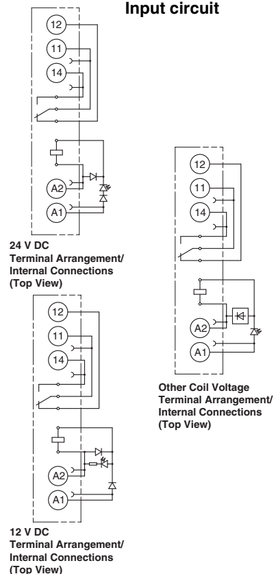
Terminal Arrangement
