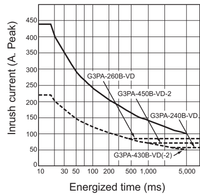
G3PA-240B-VD/G3PA-260B-VD, G3PA-430B-VD, G3PA-430B-VD-2, G3PA-450B-VD-2
