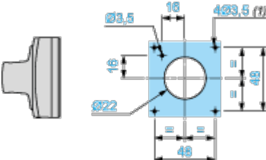
Door cut-out
