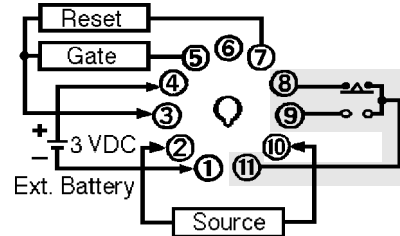
H5CN-□□□M Timer
