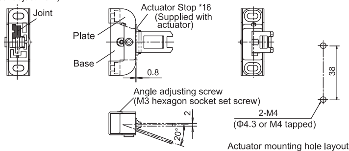
Actuator mounting hole layout
