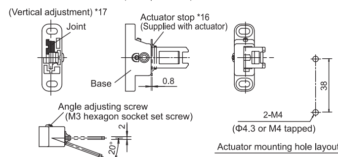
Actuator mounting hole layout
